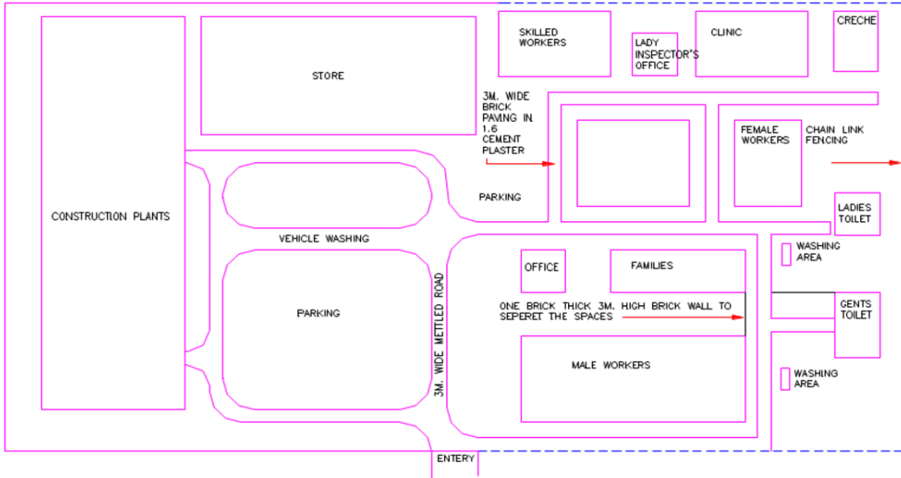
Schematic Drawing of Construction Camp
